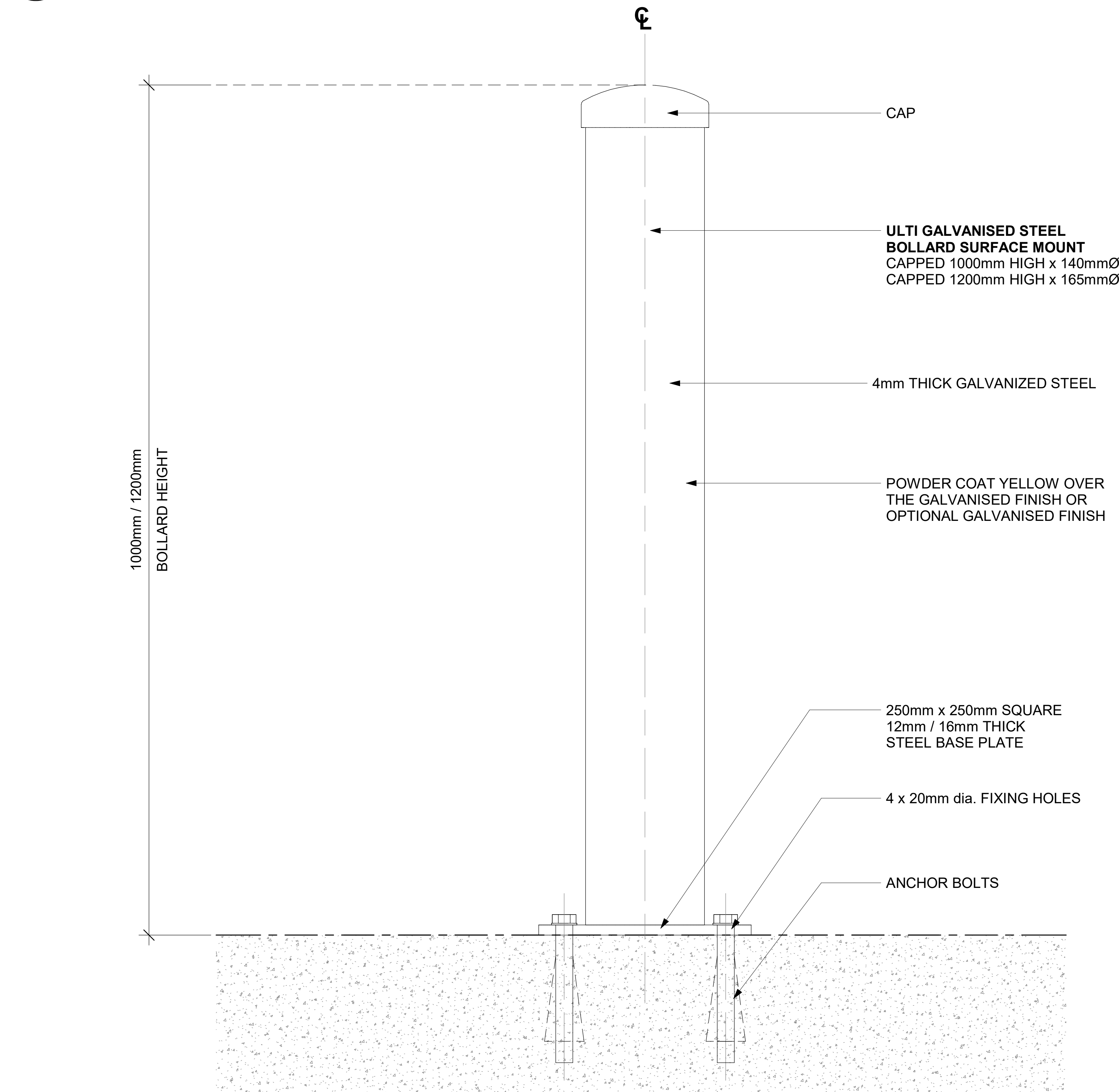
2 ELEVATION - SURFACE MOUNT BOLLARD
