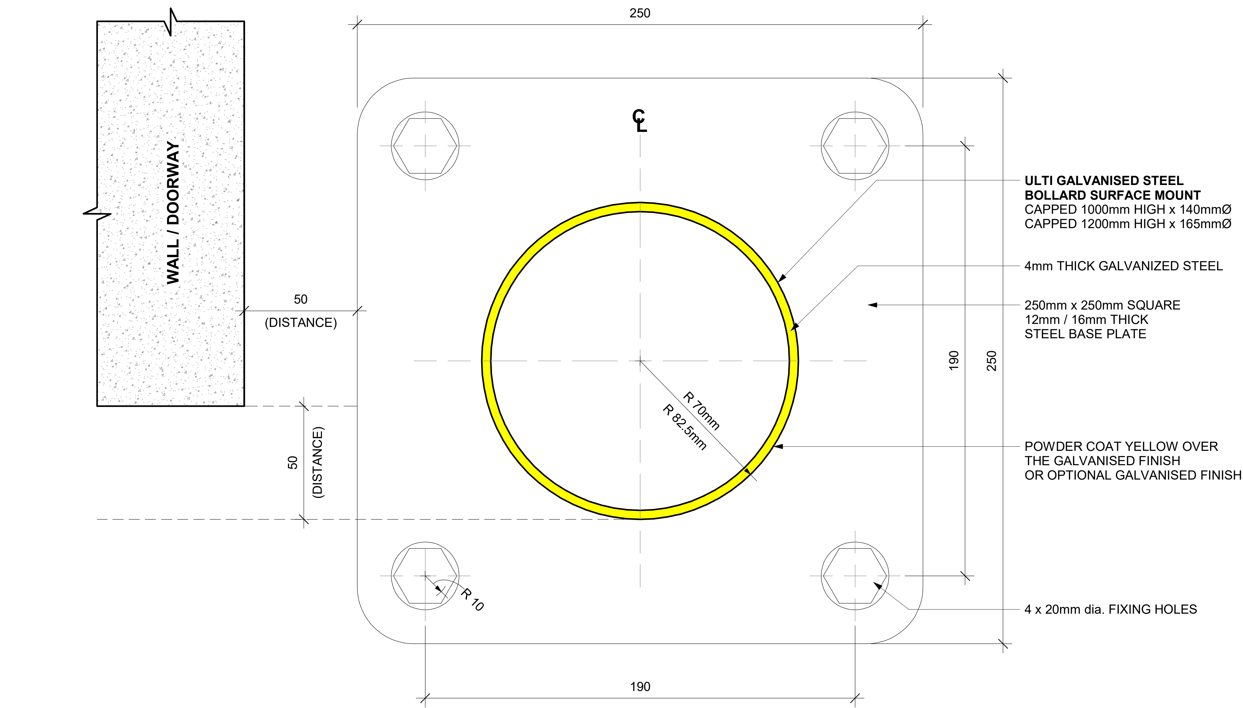
1 PLAN - SURFACE MOUNT BOLLARD
